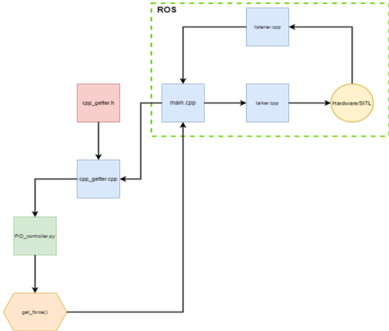
Fig. 4 Integrating a PID Controller to control a quadrotor's x-position.
