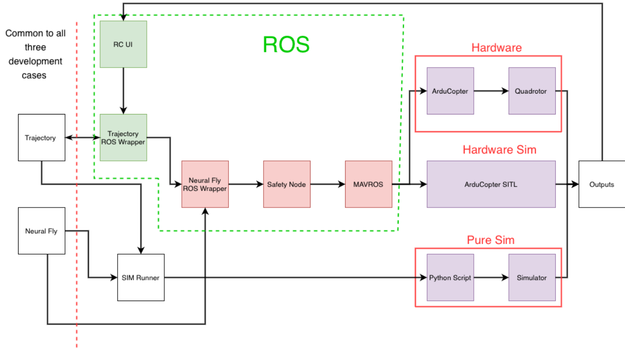
Fig. 1 Neural Fly Code Diagram. I am working on the Neural Fly ROS wrapper so the simulator can interface with the SITL and hardware.
