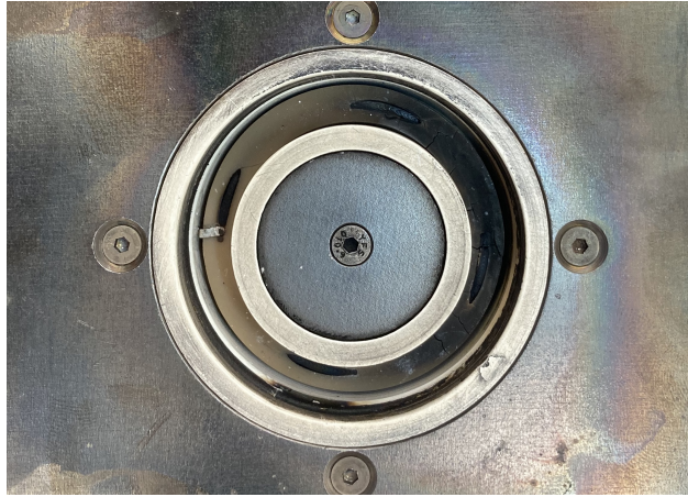
Fig. 7 Photograph of the thruster with the anode plate removed. Charring and thermal damage (right) is exactly opposite the side of the diffuser which accommodates a wire (left) used to close the electrical connection to the anode.
