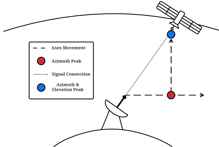
Fig. 2 Step Tracking Finding Signal Peak Along Azimuth and Elevation Axes.
