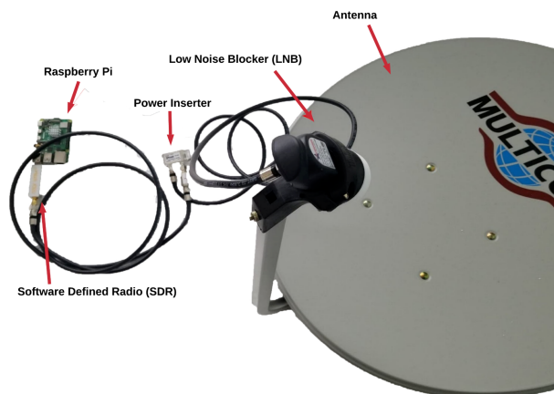
Fig. 12 Annotated Photo of the Dish-to-Raspberry Pi Setup
