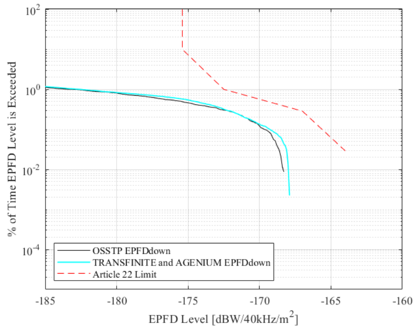
Fig. 13 Validation of METHERA-A's EPFDdown Compliance This run used a satellite frequency of 17.8 GHz, a dish size of 1m, FSS, and a reference bandwidth of 40kHz.
