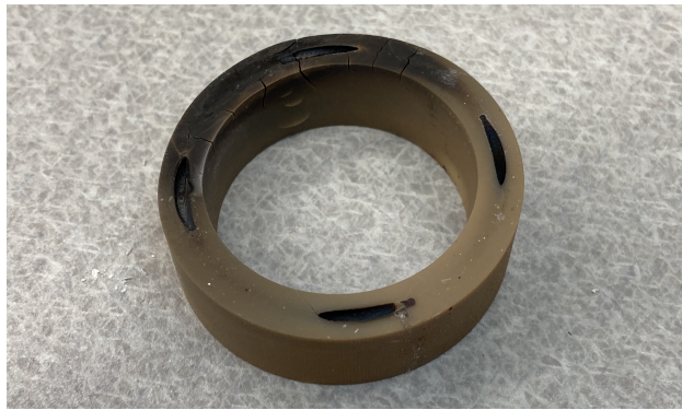
Fig. 6 Photograph of the diffuser post-firing.
