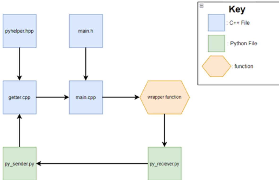
Fig. 3 Code architecture to integrate Python and C++
