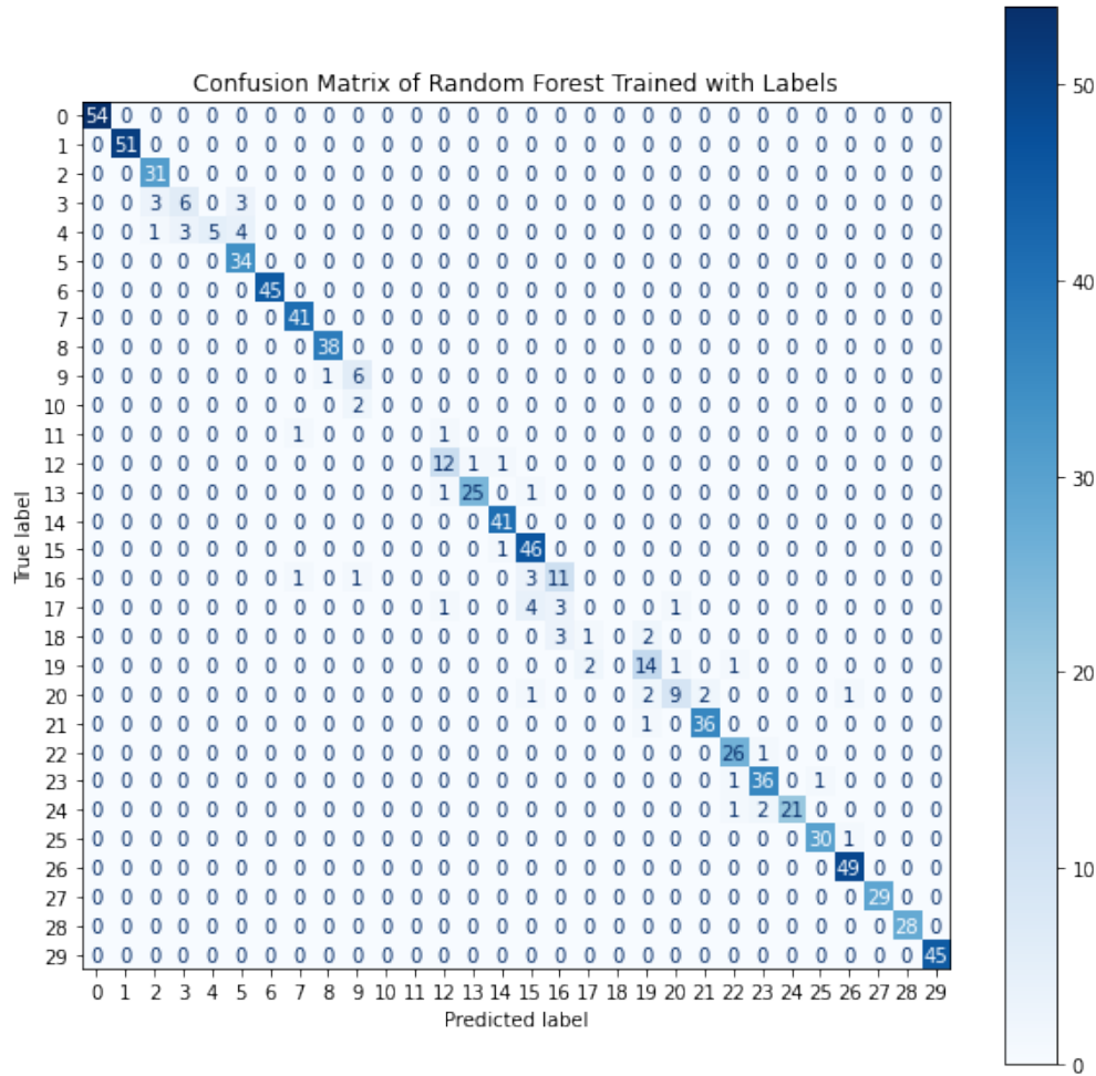
Fig. 2 The confusion matrix from a random forest trained with the location labels present in the training set. This forest has an accuracy of 92.5% at identifying craters in the test set and the high accuracy is visible in the diagonal line across the matrix. The Y-axis of the confusion matrix shows the true location of each crater while the X-axis shows the location predicted by the random forest. Each integer label corresponds to a USGS quadrangle.
