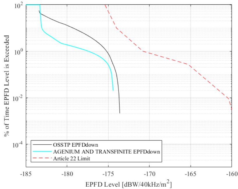
Fig. 14 Validation of 3ECOM-1's EPFDdown Compliance. This run used a satellite frequency of 10.7 GHz, a dish size of 0.6m, FSS, and a reference bandwidth of 40kHz.
