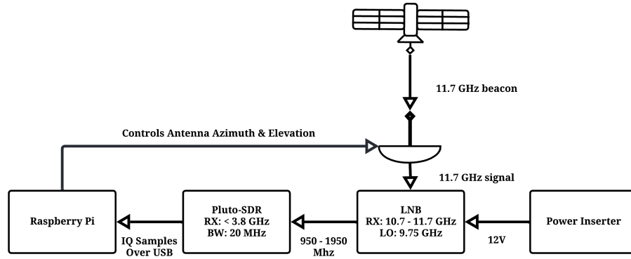
Fig. 3 Radio Signal Pre-Processing
