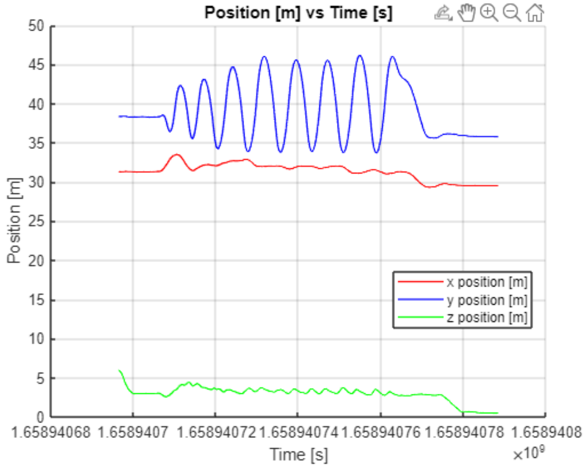
Fig. 8 Position of the quadrotor in the xyz directions [m] vs time [s]. The time is the seconds since unix epoch, January 1, 1970
