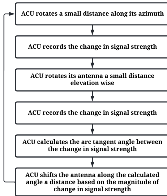
Fig. 4 Modified Step Tracking Process Steps
