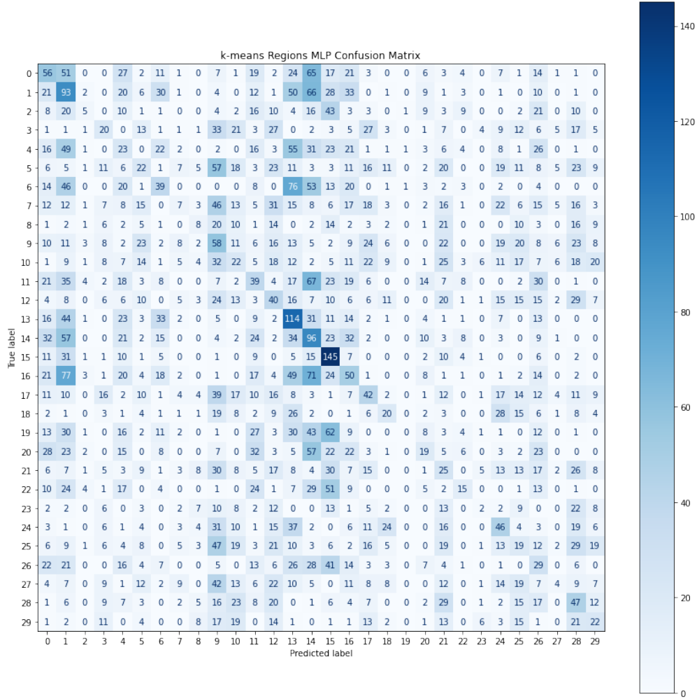
Fig. 5 The confusion matrix for the multi-layer perceptron using crater data categorized into regions found by k-means clusters. Overall accuracy is lower and the confusion is more diffuse across the whole matrix, but region 15 seems to stand out as one that is guessed most often. This region happens to be the Sea of Tranquility.
