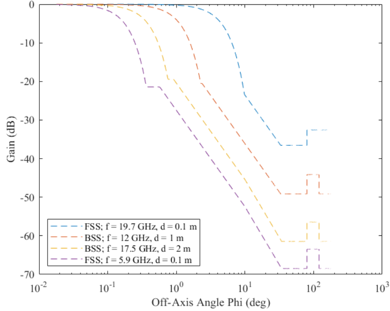
Fig. 11 Examples of Gain Patterns as a function of frequency, GSO ES Antenna Diameter, and service class: fixed-satellite service (FSS) or broadcasting-satellite service (BSS)
