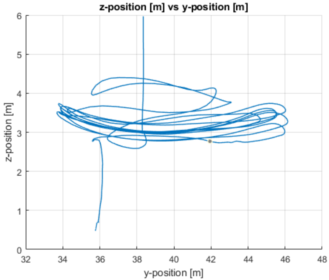
Fig. 9 Position of the quadrotor in the z-direction [m] vs the position of the quadrotor in the y-direction [m]. While the figure 8s are not perfect, the quadrotor is following a path like a figure 8
