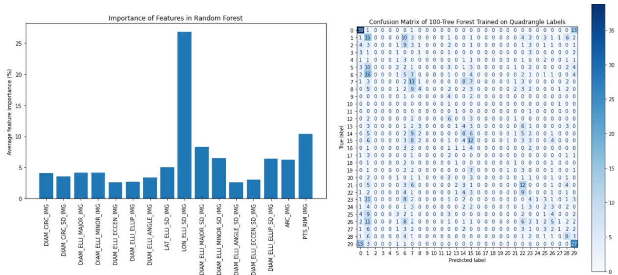
Fig. 3 (Left) The 16 crater features used for training and their relative importance in a random forest of 100 decision trees. Each tree has its own weighting of feature importance; this graph shows the average importance of each feature, taken as an arithmetic mean across all 100 trees in the forest. (Right) The confusion matrix for the same forest. This random forest has a classification accuracy of 19.25%. Higher numbers of predicted craters are represented by darker squares. The true location is shown on the y-axis and the predicted on the x-axis. A perfect prediction would result in a diagonal line from top left to bottom right; the faint diagonal line in this figure is an indicator of the algorithm's successes.
