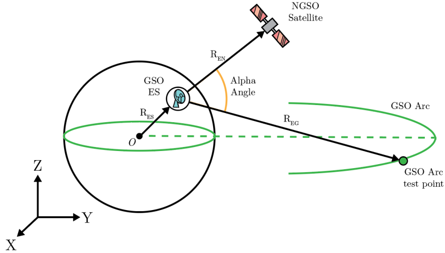
Fig. 6 Diagram of the Alpha Angle
