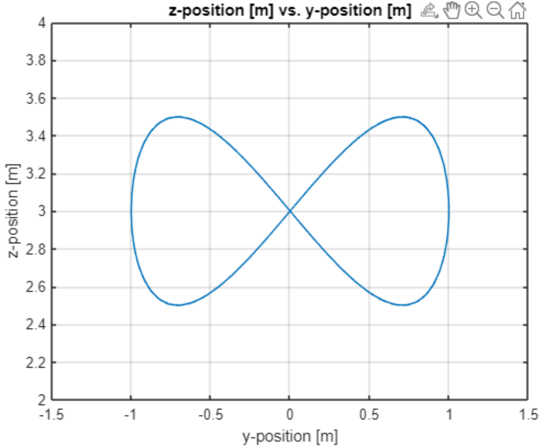
Fig. 7 Planned Flight Path for SITL testing and Hardware testing. I decided to fly in a vertical figure 8 formation to check altitude control. The parametric equation for this plot was: x(t) = 0 , y(t) = \sin(t) , z(t) = \sin(t)\cos(t) + 3
