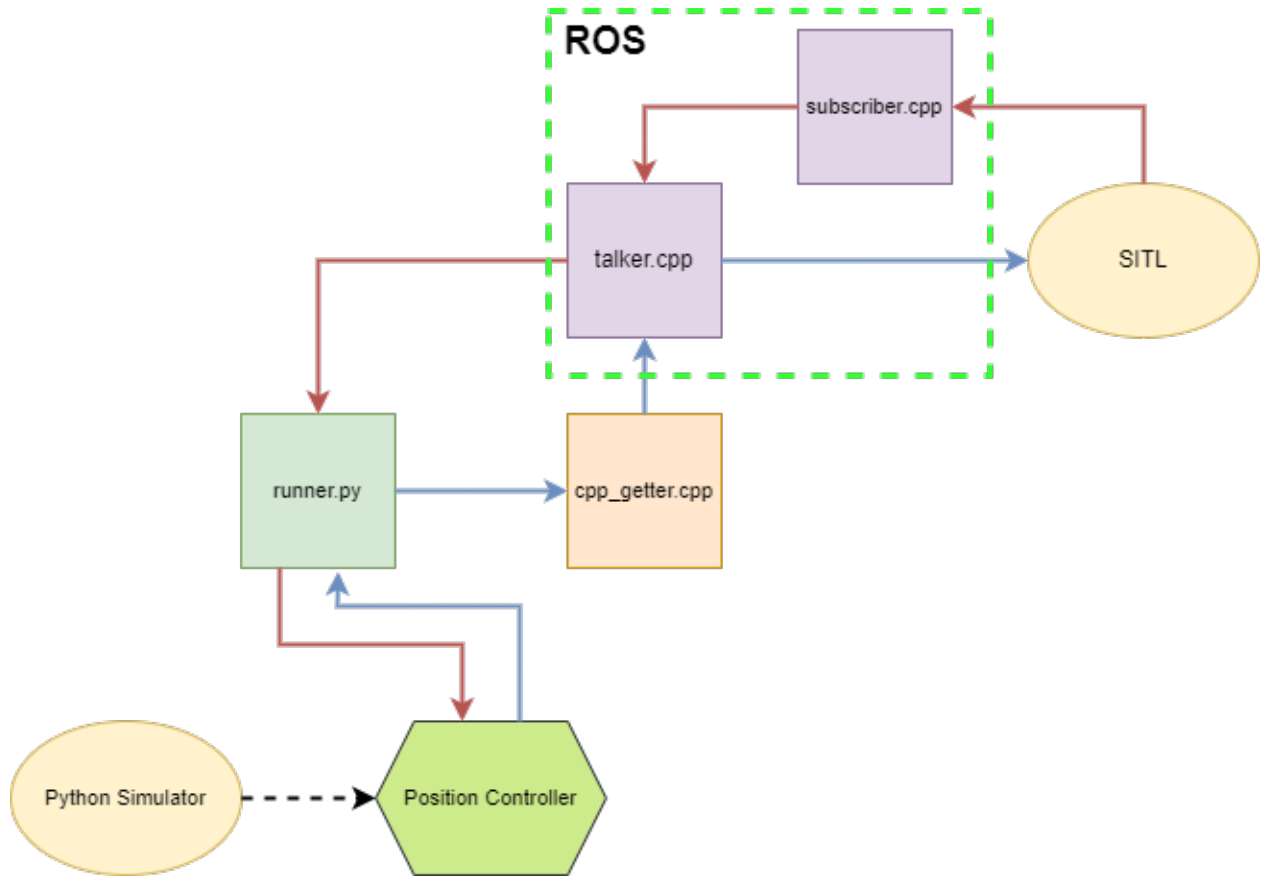
Fig. 5 Controller Integration. The path the data from the quadrotor follows is indicated by red arrows, and the path the returns follows is indicated by blue arrows. The main elements I developed are the non-ROS parts of the talker node, the C++ getter file ( cpp_getter.cpp ), and the python script, runner.py .
