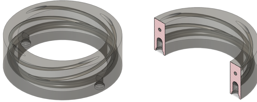
Fig. 1 CAD model and section view of the diffuser used during testing. This figure by Braden Oh, et al. [3] is licensed under CC BY 4.0.
