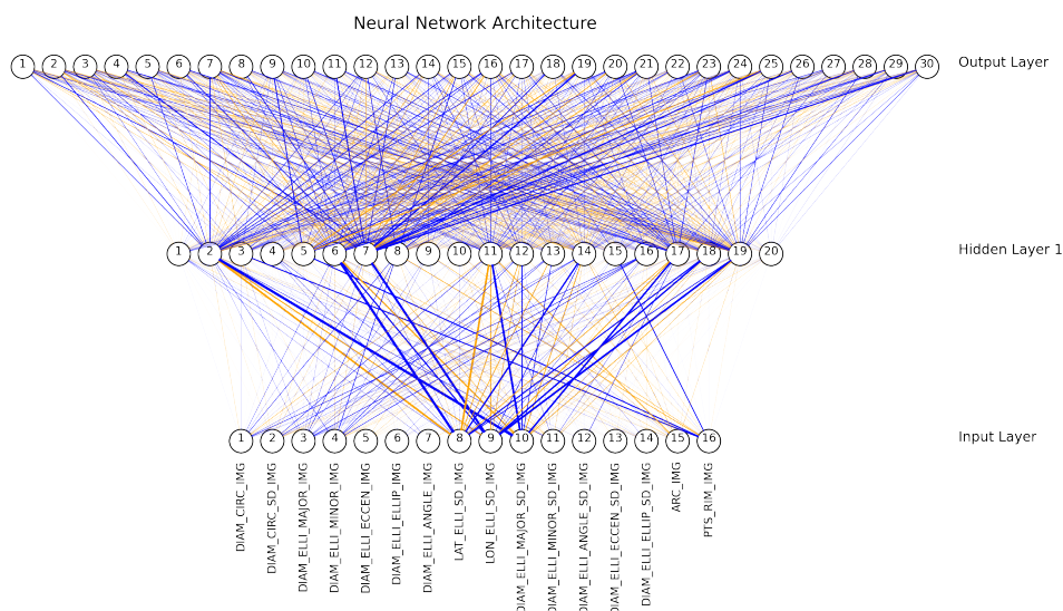
Fig. 7 The network structure for the MLP trained on k-means cluster data. Created with Liu [11].
