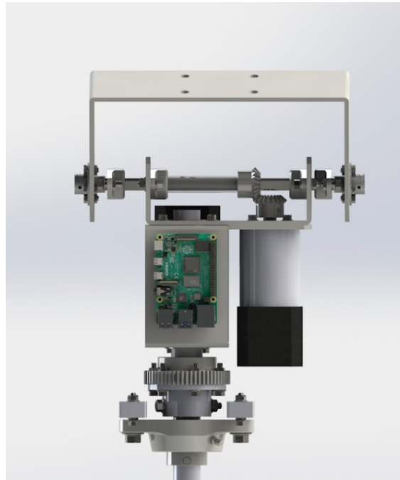
Fig. 8 Rendering of Mechanical System
