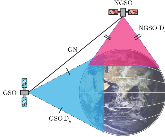
Fig. 4 Diagram of Visible Systems
