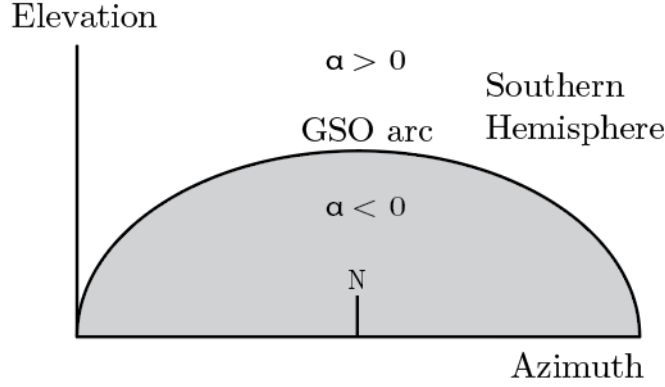
Fig. 9 Sign of \alpha given R_{z=0} with respect to R_{GEO} in the Southern Hemisphere looking North
