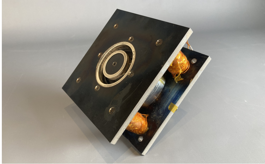
Fig. 3 A post-firing photograph of the thruster used to test the diffuser.
