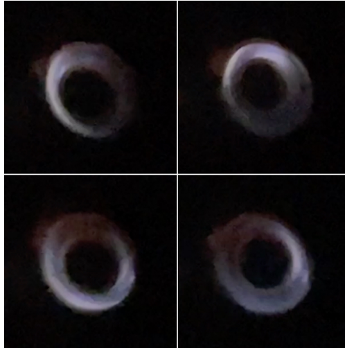
Fig. 5 Still frames from video of a clockwise-rotating spoke instability.
