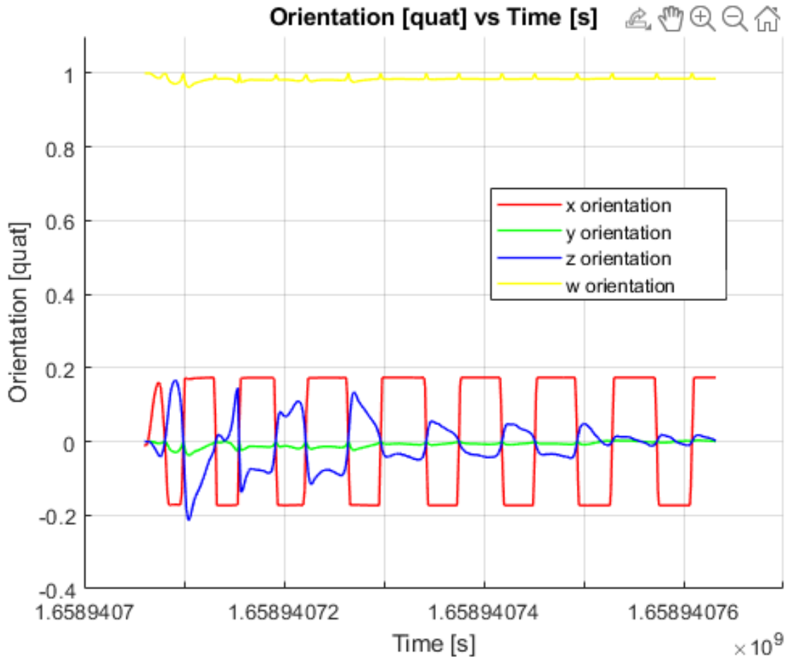
Fig. 10 Orientation of the quadrotor [quat] vs time [s]
