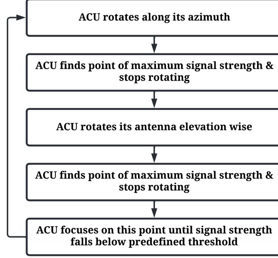
Fig. 1 Main Stages of the Step Tracking Process.
