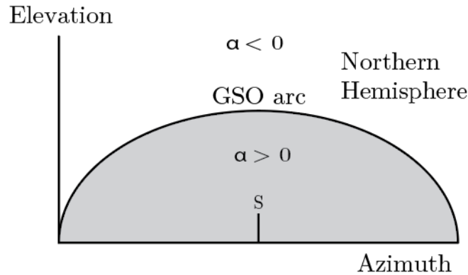
Fig. 8 Sign of \alpha given R_{z=0} with respect to R_{GEO} in the Northern Hemisphere looking South
