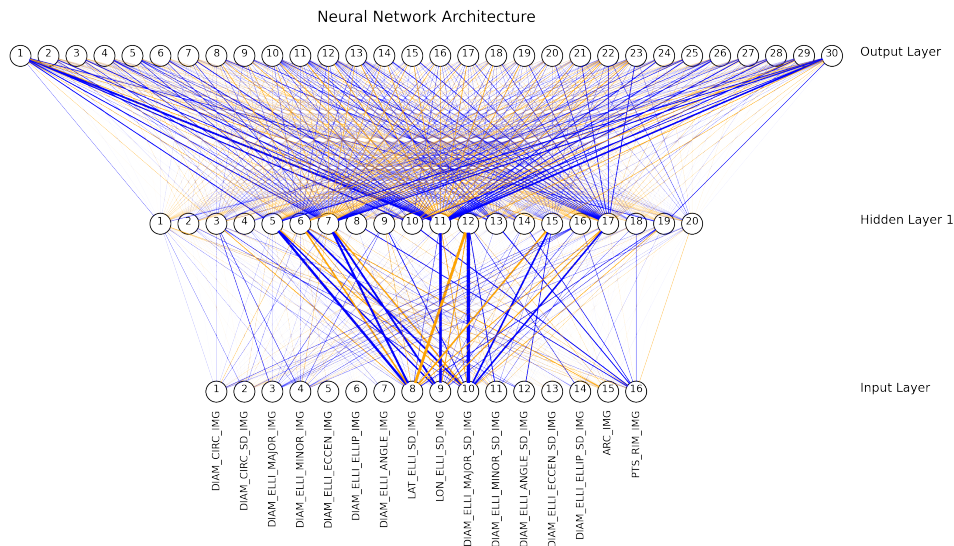
Fig. 6 The network structure for the MLP trained on USGS quadrangle data. Blue weights are positively-valued, and orange weights are negatively-valued. The size of the lines representing each weight indicate their relative weighting. From the strong weights associated with LAT_ELLI_SD_IMG, LON_ELLI_SD_IMG, and DIAM_ELLI_MAJOR_SD_IMG, we infer that these parameters are most important for classification. Created with Liu [11].
