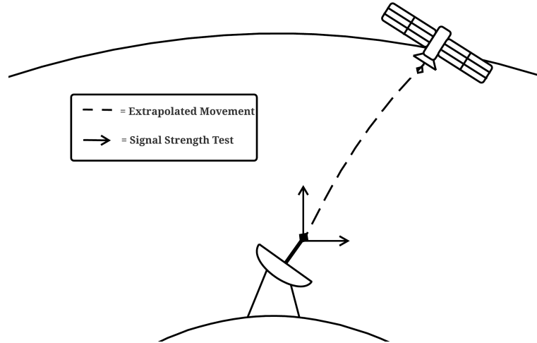
Fig. 6 Modified Step Tracking Function Testing Signal Strength Difference in Two Axes Before Extrapolating an Orientation Trajectory
