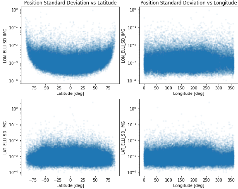
Fig. 8 Plots of position standard deviation vs position for ellipse fits. Longitudinal standard deviation increases near the poles because the degree error per unit distance at high latitude is greater than the degree error near the equator. The classifiers both identified this as a way to recognize polar craters.
