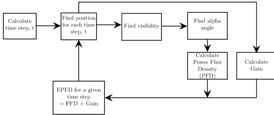
Fig. 3 Block diagram of the EPFDdown Validation Algorithm
