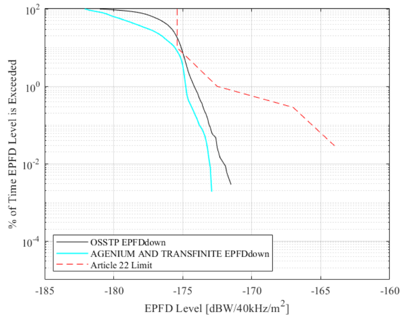
Fig. 12 Validation of ARISTARCHUS's EPFDdown Compliance. This run used a satellite frequency of 17.8 GHz, a dish size of 1m, FSS, and a reference bandwidth of 40kHz.
