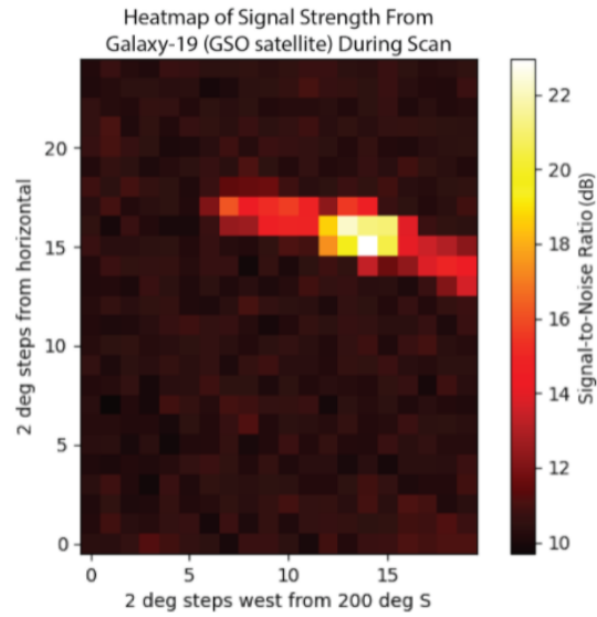
Fig. 9 A Heat Map of a Sample Scan for the Galaxy-19 GSO Satellite
