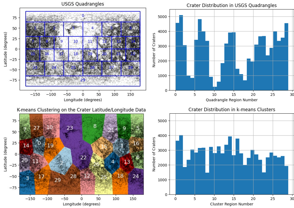
Fig. 1 (Top left) Map of lunar crater positions with USGS quadrangle overlay. Crater centers plotted with 10% transparency. (Top right) Distribution of lunar craters in USGS quadrangle regions. This distribution could bias the algorithms to classify craters into certain regions simply because they have more craters. If this bias is present, regrouping our data more evenly would significantly change the error rate. (Bottom left) Map of lunar crater positions regrouped by k-means clustering. Crater centers also plotted with 10% transparency. (Bottom right) Distribution of lunar craters in 30 k-means regions. These regions are more evenly distributed and consistently produce higher error rates than the USGS regions.
